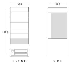
FROST TECH SD60-60HC H 1950mm W 600mm D 600mm
