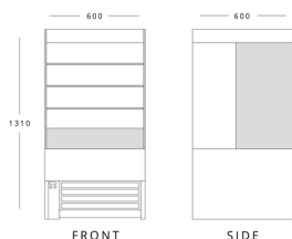
FROST TECH SLD60-60HC H 1310mm W 600mm D 600mm
