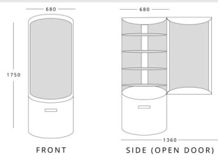
BLIZZARD CD400R H 1750mm W 680mm D 680mm
