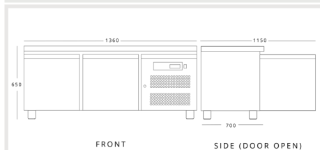
BLIZZARD SNC2 H 650mm W 1360mm D 700mm
