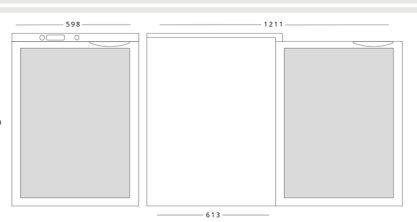
BLIZZARD GF140 H 819mm W 598mm D 613mm
