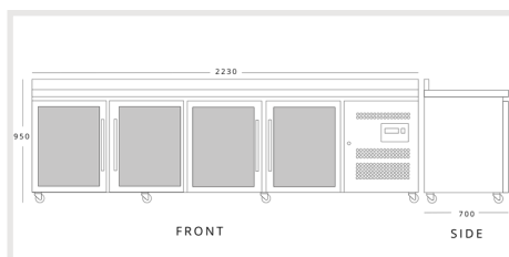
BLIZZARD HBC4CR H 950mm W 2230mm D 700mm
