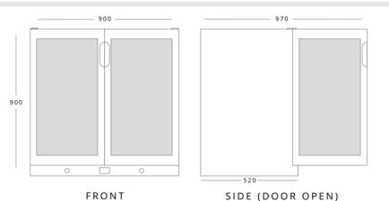
INFRICO ZX2(SS) H 900mm W 900mm D 520mm
