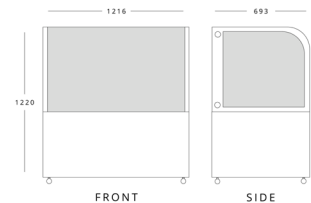
BLIZZARD DC370 H 1220mm W 1216mm D 693mm
