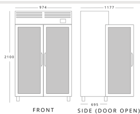
INFRICO AGN602-CR H 2100mm W 482mm D 695mm
