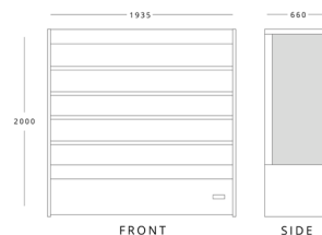
BLIZZARD BTD200WH (SS,BK) H 2000mm W 1935mm D 660mm
