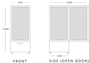
BLIZZARD CD400L H 1908mm W 650mm D 650mm
