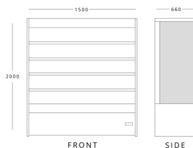
BLIZZARD BTD150WH (SS,BK) H 2000mm W 1500mm D 660mm
