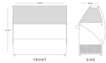
CRYSTAL ELEGANTE46 H 1257mm W 1447mm D 824mm
