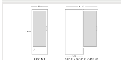
INFRICO ZX10(SS) H 1800mm W 600mm D 520mm
