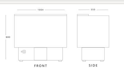
INFRICO EFP1000SS(WH) H 880mm W 1004mm D 550mm
