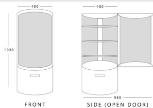
BLIZZARD CD100R H 1030mm W 480mm D 480mm
